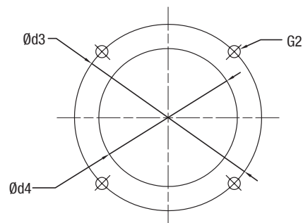
Mounting Detail
