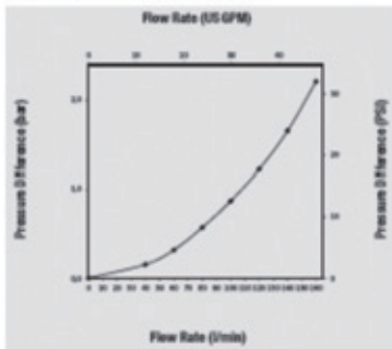
Series FF 18 • BG 6 • Nominal Size 18
