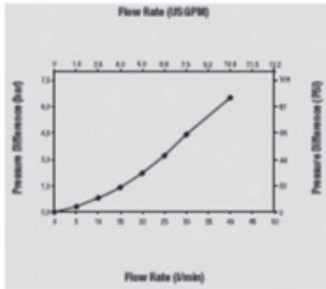
Series FH 06 • BG 1 • Nominal Size 6,3
