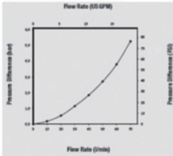
Series FF 10 • BG 2 • Nominal Size 10
