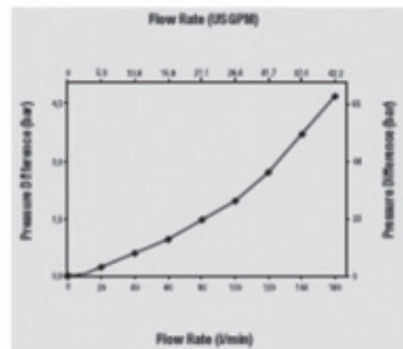
Series FH 16 • BG 4 • Nominal Size 16
