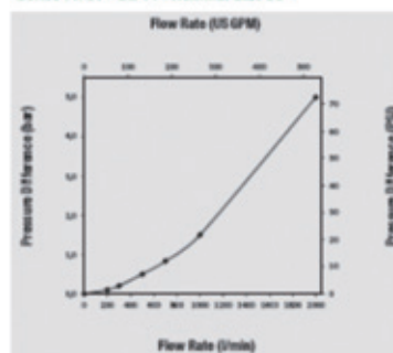
Series FH 51 • BG 14 • Nominal Size 50
