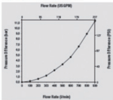
Series FX 38 • BG 12 • Nominal Size 31,5
