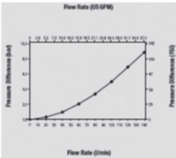
Series FU 12 • BG 3 • Nominal Size 12
